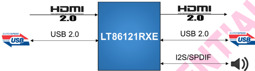
Figure 3.1 Application Diagram
